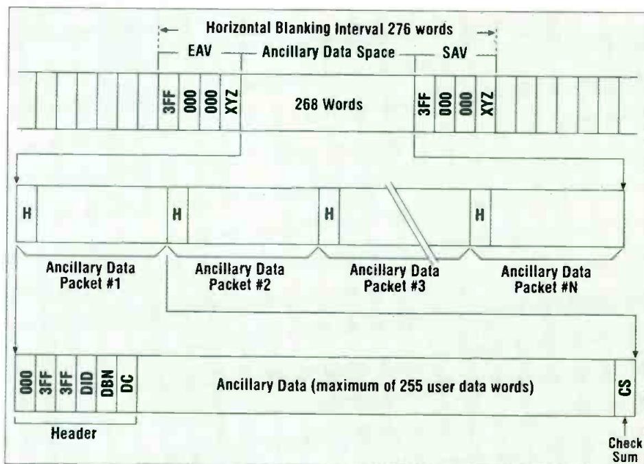
Figure 2: Ancillary data packets within the horizontal blanking interval consist of a 6 byte header, up to 255 user data words and a checksum word.
